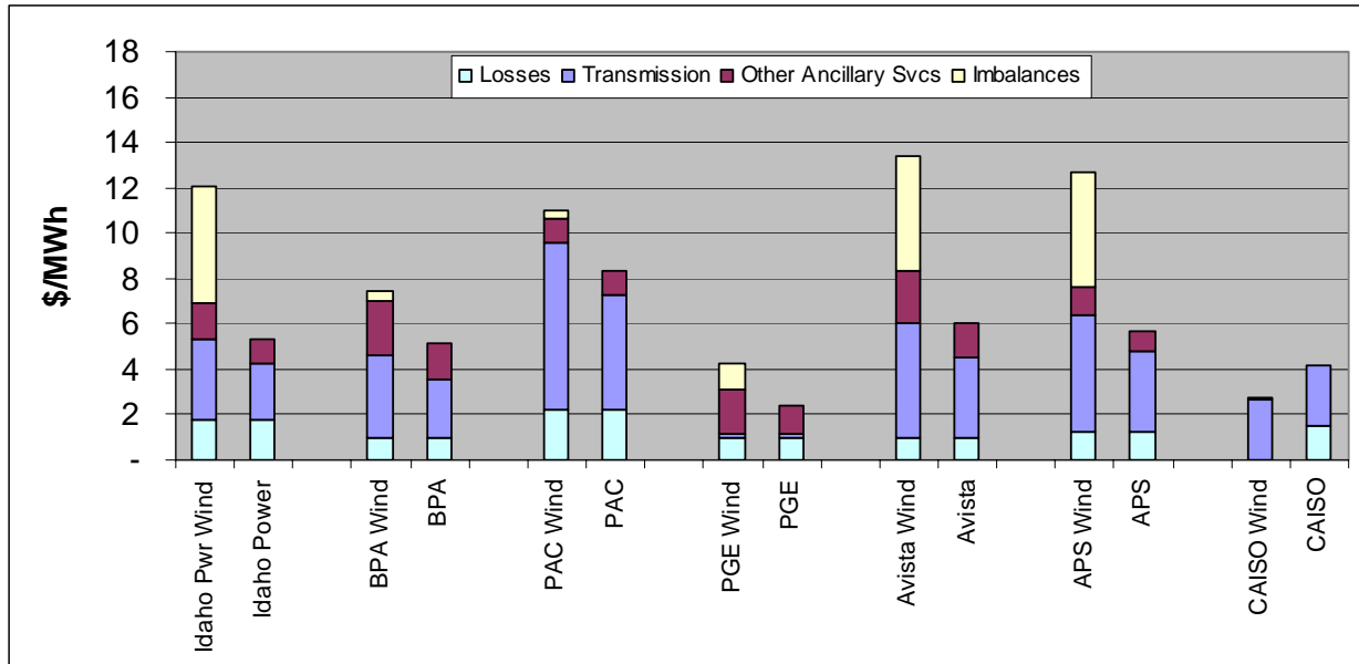
Figure 3: Cost Comparison of Transmission for Wind vs. CCGT Plants
